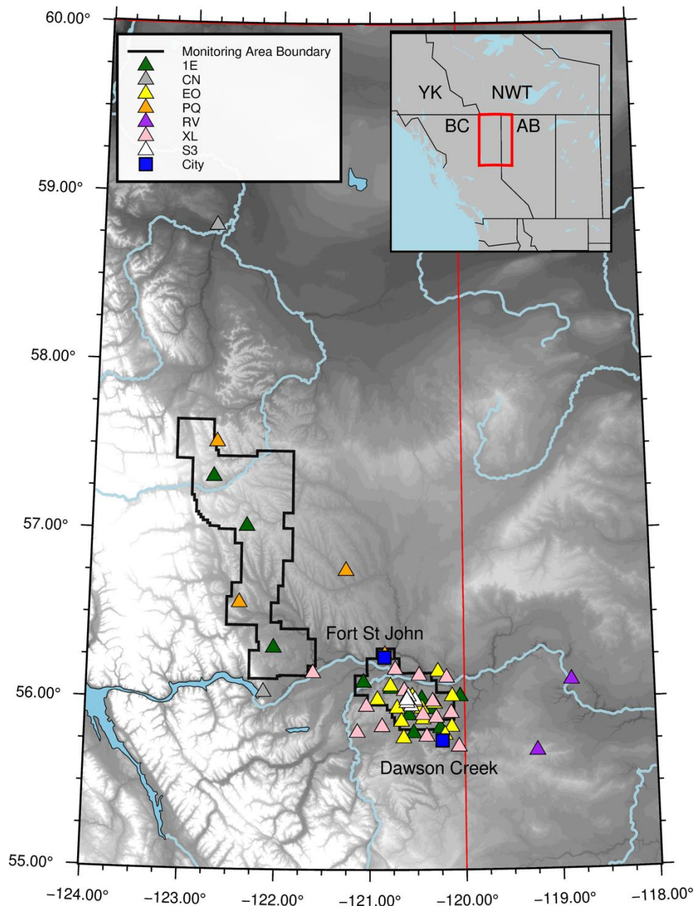
Figure 1. Stations used to locate events in NE BC from April 1, 2021, to May 1, 2022.
