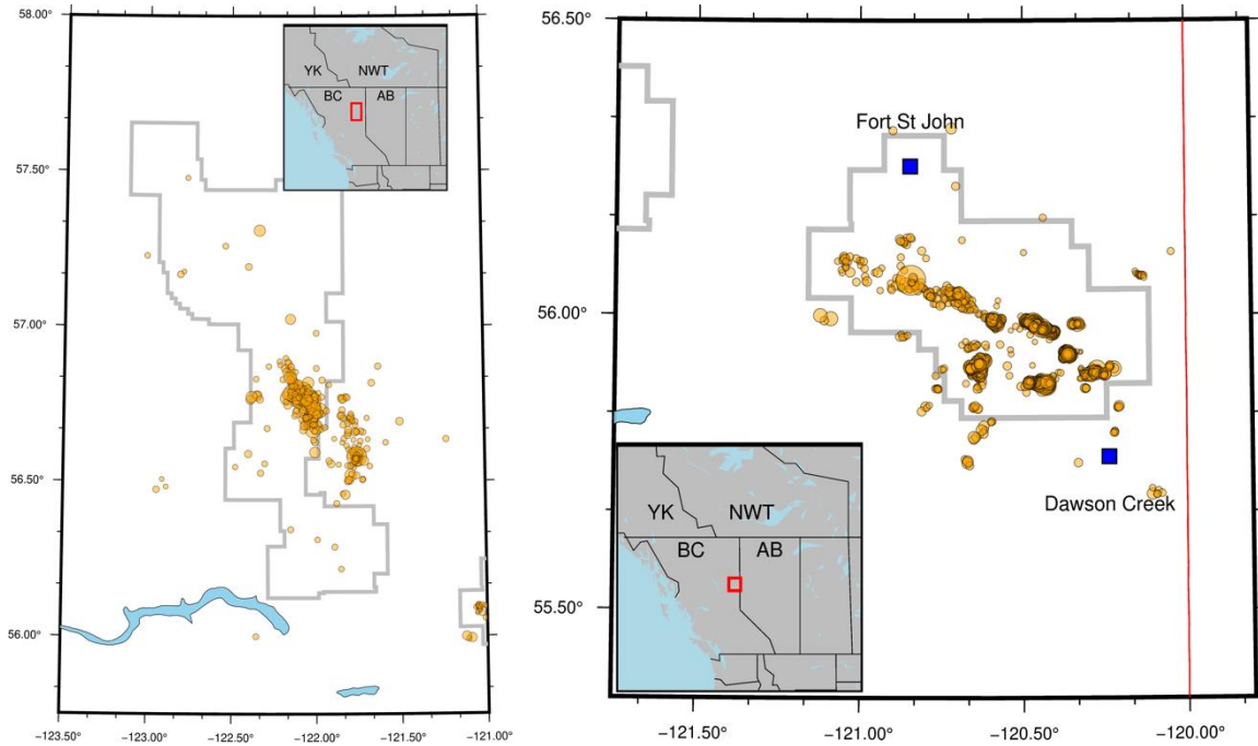
Figure 3. Seismicity occurring in NE BC in the NM (left) and the KSMMA (right).
