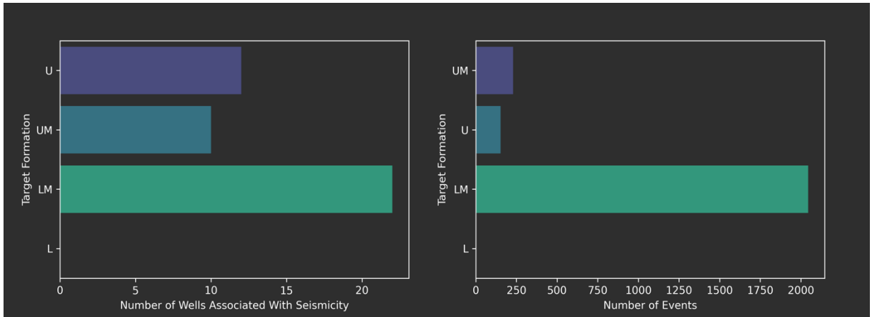
Figure 7. Number of hydraulic fracturing wells associated with seismicity by their target formation in the KSMMA (left). Number of events associated with wells by well target formation in the KSMMA (right). Data presented is using all available data as of May 1 st , 2022.
