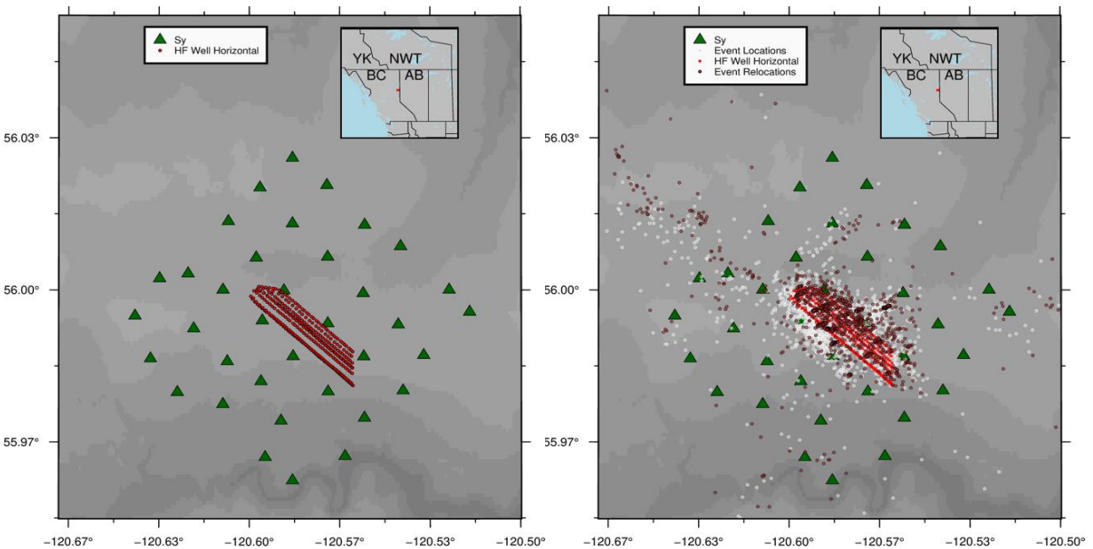
Figure 8. Symroc network stations (Sy) and the studied well pad in the KSMMA from January 1, 2021 to June 1, 2021 (left). Events located using the Symroc stations and relocated event locations from the HypoDD relocation algorithm (right).
