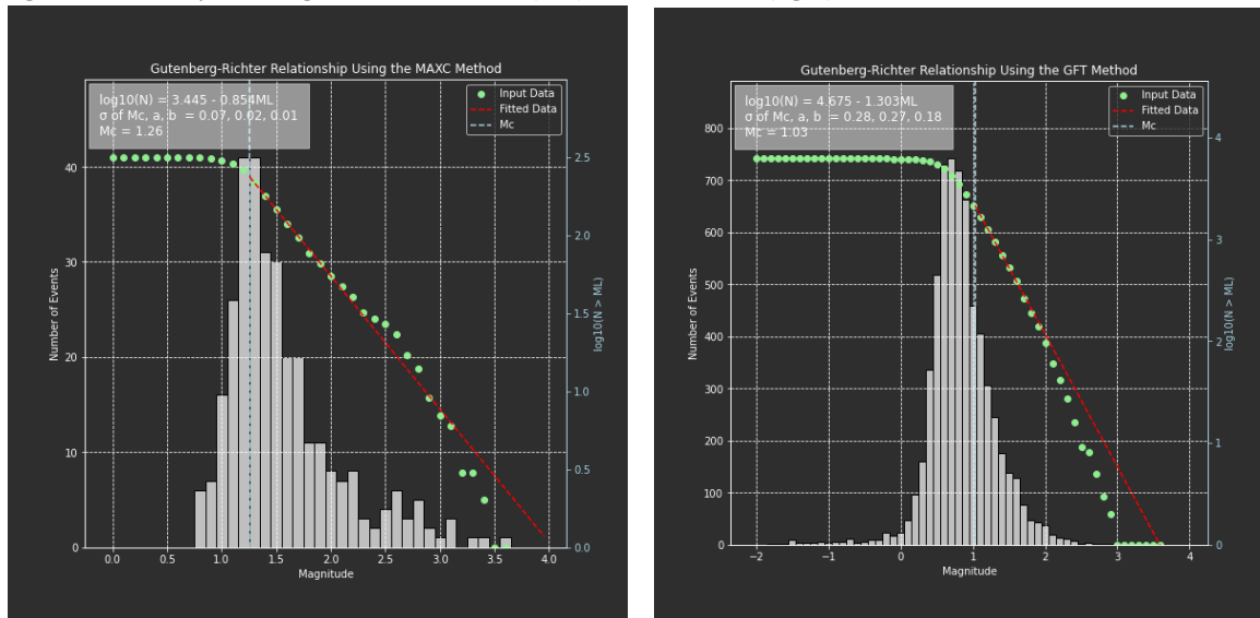
Figure 4. Magnitude of completeness in NE BC in the NM (left) and the KSMMA (right).
