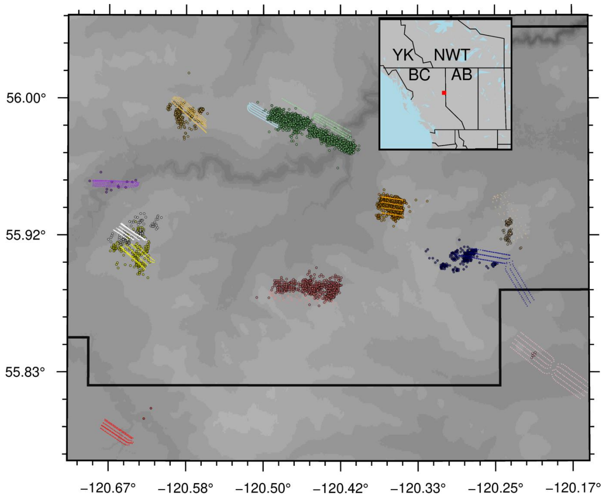
Figure 6. Events from April 1, 2021 to May 1, 2022 that have been automatically associated with hydraulic fracturing well pads within the KSMMA as of May 1 st , 2022. Associated well pads and earthquakes are shown in the same colour. Seismic events are shown with black edges while the horizontal well-paths are shown without the black edge.
