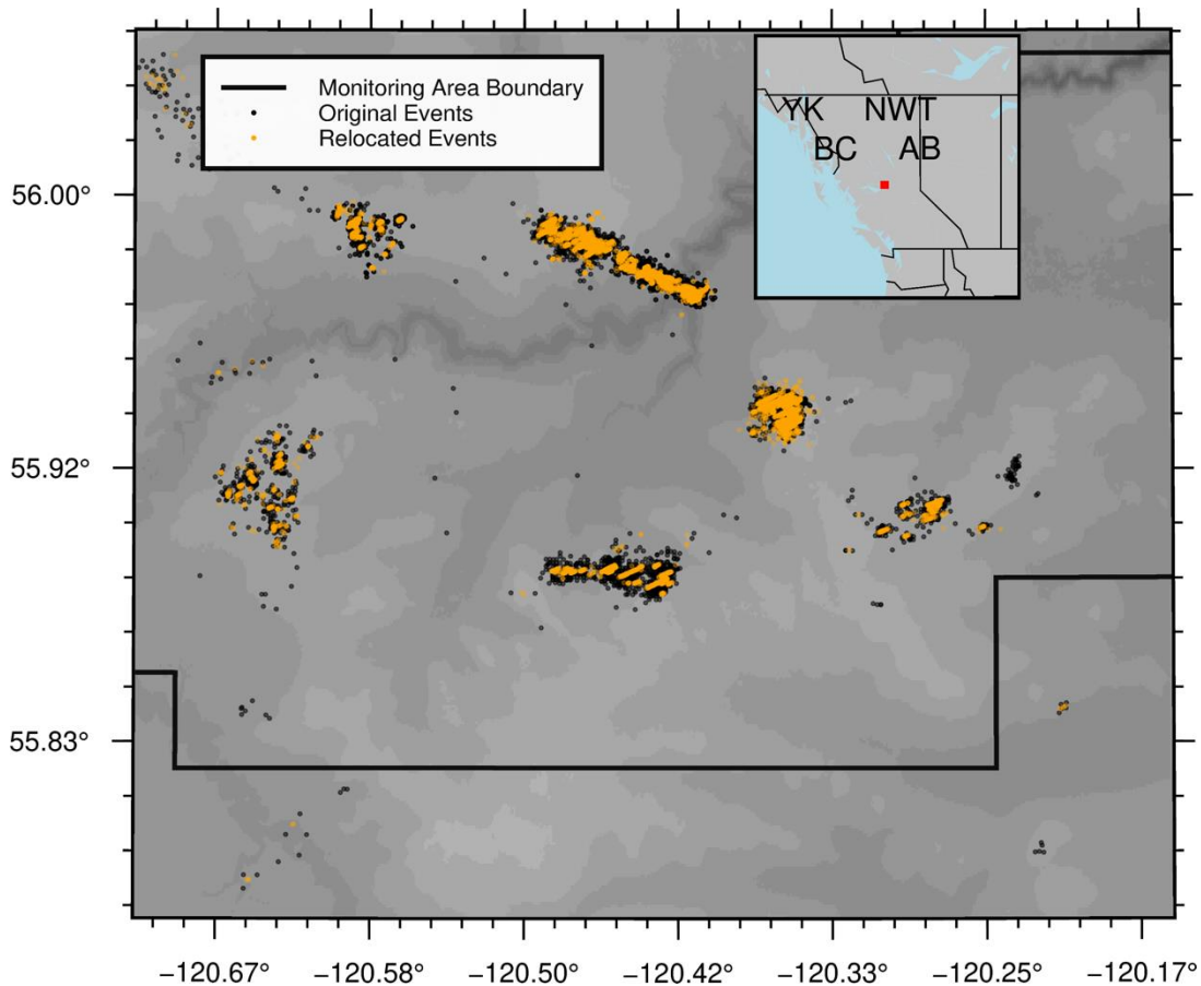
Figure 5. Original and automatically relocated earthquakes in the KSMMA as of May 1 st , 2022. Relocated events are shown in orange while the original event locations are shown in black. NE-SW trending lineations are visible in the relocated dataset.
